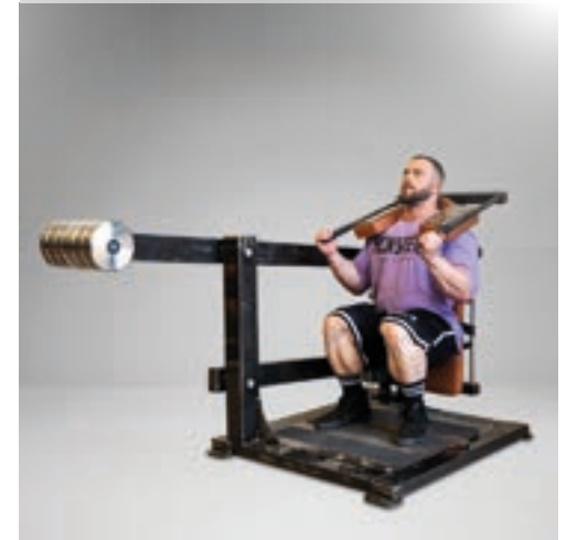
TRUSQUAT
